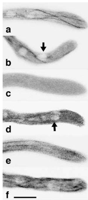
Fig. 1 Representative images of Aspergillus nidulans hyphae containing green fluorescent protein (GFP)- \alpha -tubulin visualized using confocal epifluorescence microscopy of single near-median sections. Images are shown with inverted contrast so microtubules are seen as dark lines. Hyphae were (a) untreated or treated ~30 min with (b) 0.1% ethanol, (c) 1 \mu\text{g}/\text{ml} benomyl in 0.01% ethanol, (d) 5 \mu\text{g}/\text{ml} latrunculin B in 0.02% ethanol, (e) 0.25% dimethyl sulfoxide (DMSO), (f) 50 \mu\text{M} taxol in 0.25% DMSO. Some treatments, including taxol, give the impression of inducing microtubule bundling, but individual microtubules cannot be resolved with fluorescence microscopy. Arrows in b and d indicate the position of the most-apical nucleus. Bar in f = 5 \mu\text{m} , for all images
