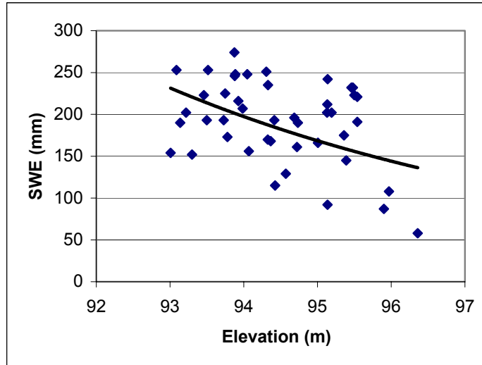
Figure 10. 2001 subalpine (depression) snow water equivalent.
