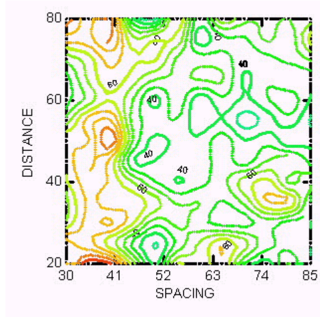
Figure 3. 2001 forest snow water equivalent.
