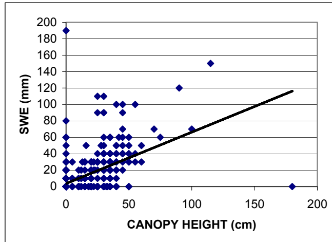
Figure 14. Alpine canopy height vs. snow water equivalent.
