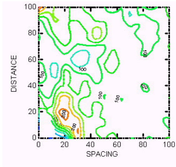
Figure 8. 2001 subalpine snow water equivalent.
