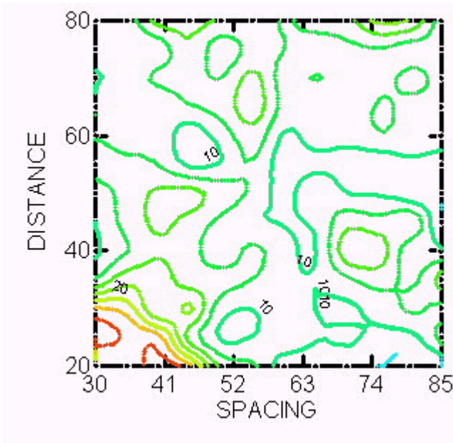
Figure 2. 2000 forest soil moisture.
