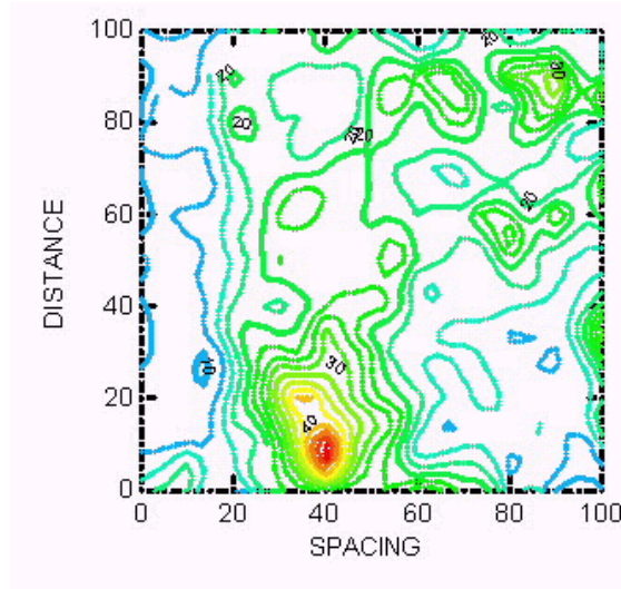
Figure 7. 2000 subalpine soil moisture.
