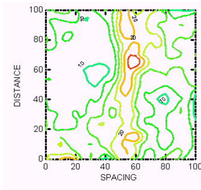
Figure 11. 2000 alpine soil moisture.
