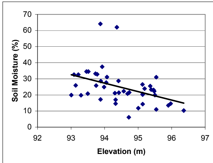
Figure 9. 2000 subalpine (depression) soil moisture.
