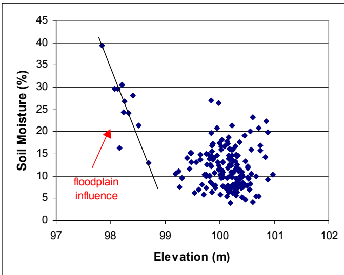
Figure 4. 2000 Forest soil moisture vs. elevation.
