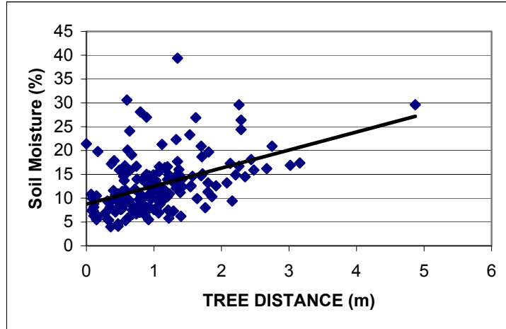
Figure 6. 2000 forest soil moisture vs. tree distance.
