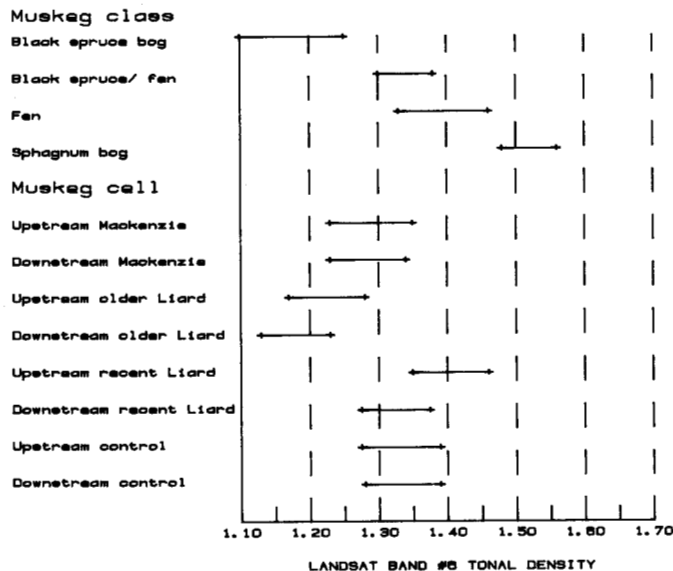
FIG. 3. Ranges of muskeg classes and cells. Ranges are based on 95% confidence intervals for means of classes and cells determined using the pooled standard deviation of classes and cells combined.
