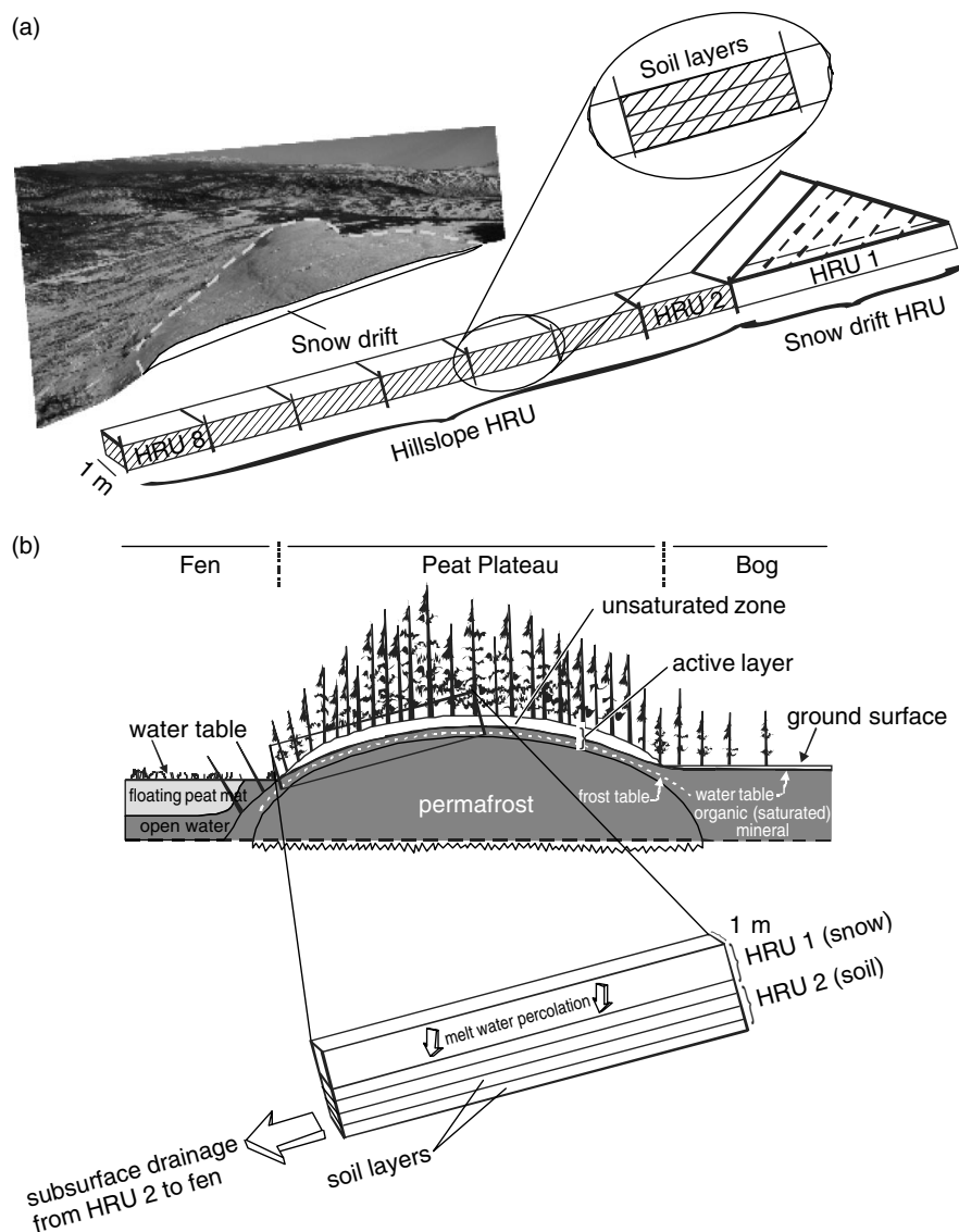
Figure 10. Contrasting configurations of HRUs for (a) the Wolf Creek Research Basin where a late-lying snowdrift is situated upslope of a series of hillslope sub-HRUs; and (b) the Scotty Creek Research Basin where peat plateau is covered by a single hillslope HRU resting below a snowpack HRU
