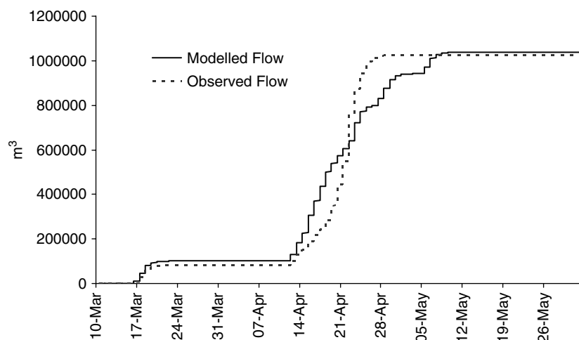
Figure 8. Cumulative measured and CRHM-modelled stream discharge, Creighton Tributary (1975)
