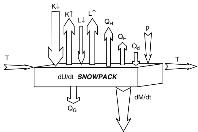
Figure 3. HRU scale control volume for snowmelt calculation. Note that T refers to horizontal transfer of snow mass which can occur due to blowing snow but is infrequent during melt. Arrows indicate direction of fluxes
