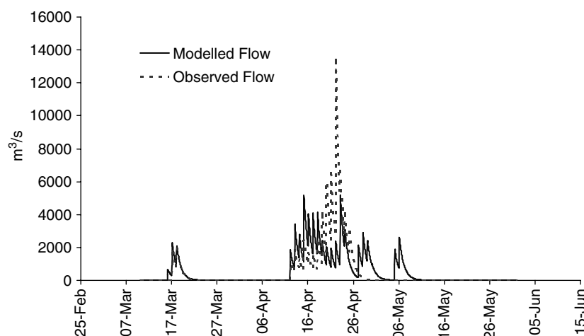
Figure 7. Hourly discharge rate in Creighton Tributary modelled by CRHM and measured, spring 1975
