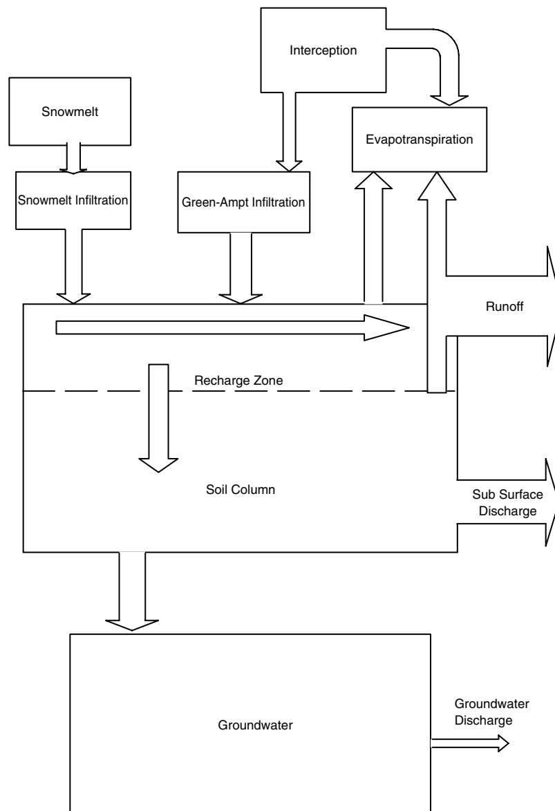
Figure 4. Flows associated with the soil moisture balance module
