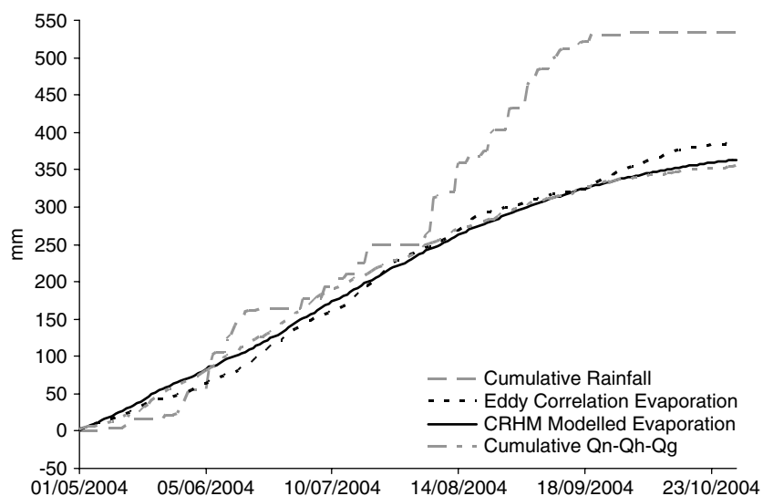
Figure 9. Modelled cumulative evapotranspiration over a fen wetland in the boreal forest of central Saskatchewan from CRHM and evaporation estimated from eddy correlation measurements and as a residual of the energy balance. Also shown is cumulative rainfall in mm
