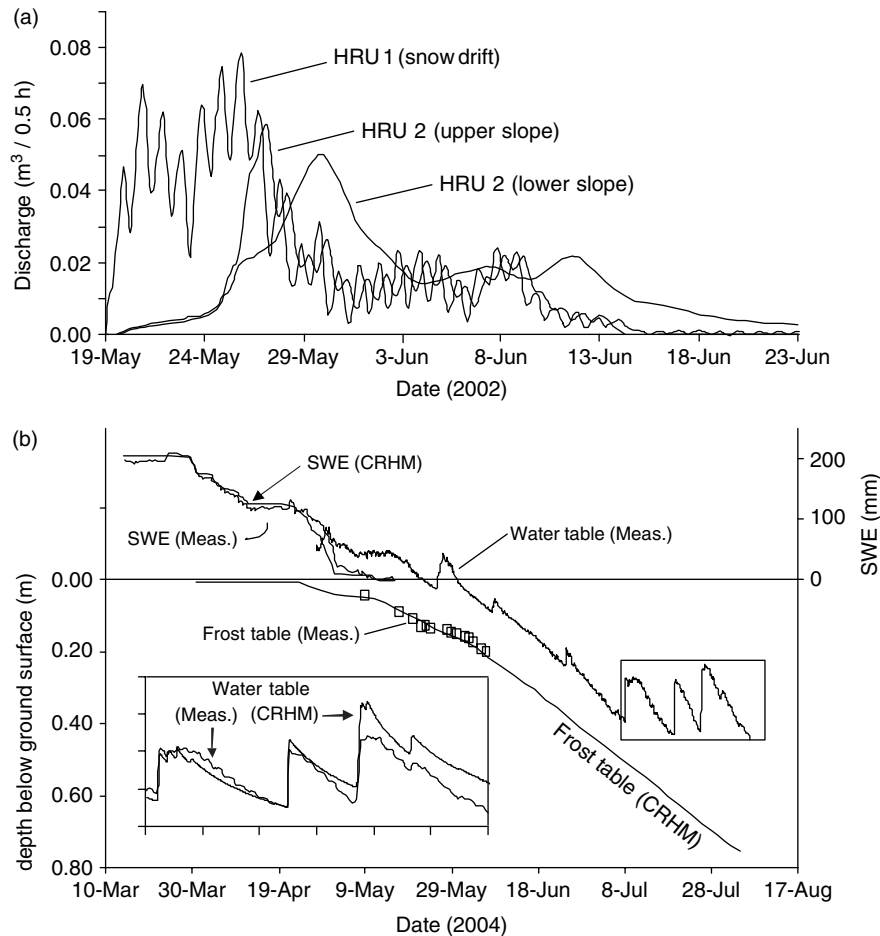
Figure 11. (a) Simulated downslope discharge from upper to lower slope positions of the hillslope HRU during the snowmelt-runoff event of 2002, north-facing slope of Granger Creek, Wolf Creek Research Basin. (b) Measured and simulated snow water equivalent depth, and depth to the frost table and water table at Scotty Creek during the snowmelt-runoff event of 2004
