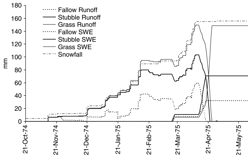
Figure 6. CRHM 'prairie' simulated SWE and runoff as mm per unit area for 3 HRU. Corrected cumulative snowfall shown for comparison. Creighton Tributary, Bad Lake, Saskatchewan
