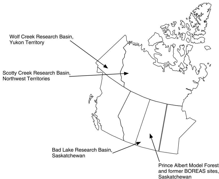
Figure 1. Locations of the research and modeling sites in western Canada. Bad Lake, Saskatchewan: semi-arid prairies, Prince Albert Model Forest/BOREAS, Saskatchewan: southern boreal forest, Wolf Creek, Yukon: sub-arctic cordilleran tundra, Scotty Creek, Northwest Territories: sub-arctic permafrost wetland
