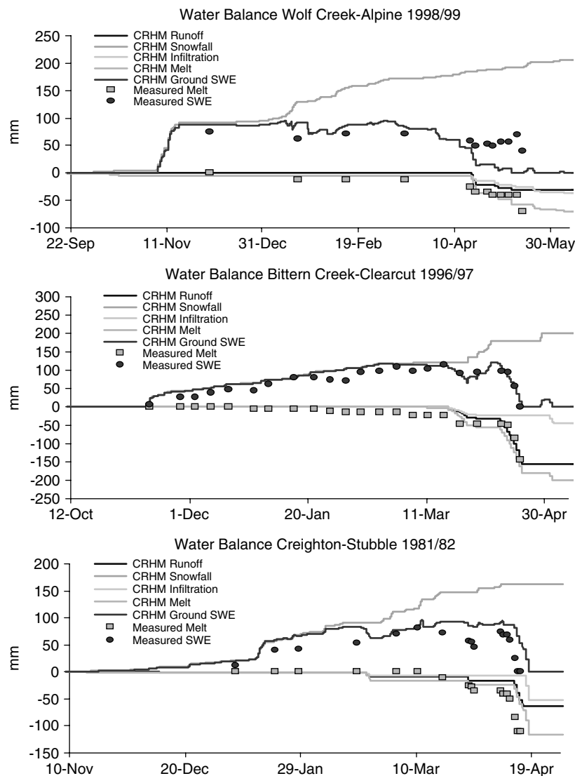
Figure 5. Simulations using the Cold Regions Hydrology Model with modules for energy balance snowmelt, blowing snow, infiltration to frozen soils, and snowmelt runoff for sites in the Prince Albert Model Forest (clear cut, Bittern Creek), Wolf Creek Research Basin (alpine ridge) and Bad Lake Research Basin (Creighton Tributary grain stubble field). Measurements of SWE and snowmelt were derived from extensive snow surveys
