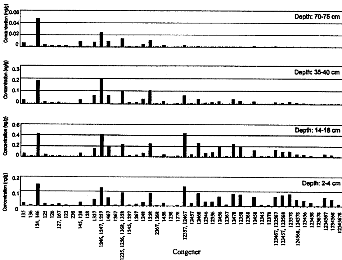
Fig. 2. Profile of PCN isomers in selected depths of a sediment core from Tokyo Bay, Japan.
