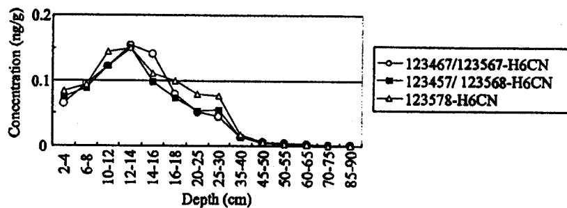
Fig. 6. Sediment core profiles of several H6CN isomers.
