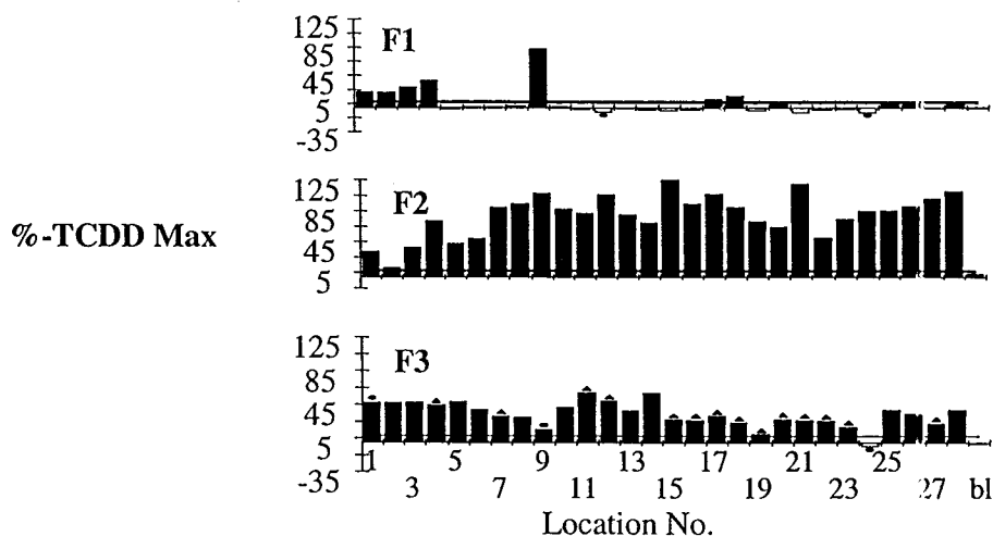
FIGURE 2. Luciferase induction in the H4IIE-luc cell bioassay (dioxin responsive) elicited by Masan Bay sediment extract fractions 1, 2, and 3 (F1, F2, F3) and procedural blank. Response magnitude presented as percentage of the maximum response observed for a 2000 pM 2,3,7,8 tetrachlorodibenzo- p -dioxin standard (%-TCDD-max.). Horizontal line equals 3 standard deviations (expressed in %-TCDD-max.) above the mean solvent control response (set to 0%-TCDD-max.). ▲ indicates cells exhibited an altered or "stressed" morphology. ● indicates the sample was toxic to the cells.
