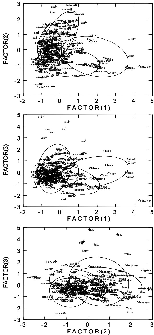
Figure 2 Overall PCA comparing 17 PCDD/F congeners in 60 On-Post and 160 Off-Post soil samples
