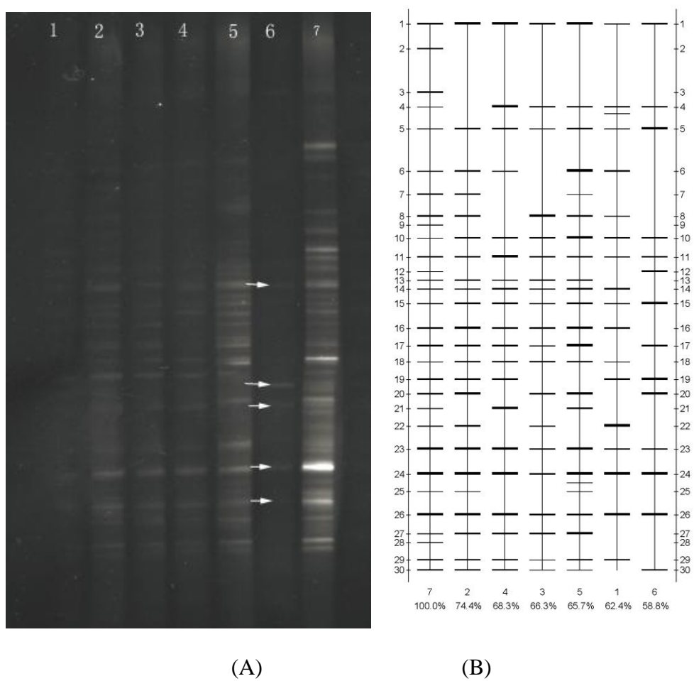
Figure 7. DGGE analysis of microbial community diversity during operation of the composting MFC process. (A) photo from DGGE analysis (B) bands simulation by quantity one.
