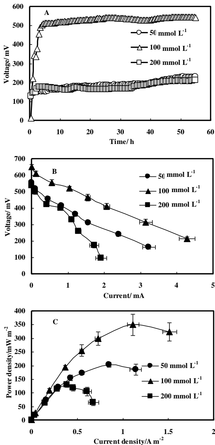
Figure 4. Effect of buffer solution on performance of the composting MFC. A: Voltage generation; B: Voltage-current curve; C: Power density curve. The error bars indicate standard deviation.
