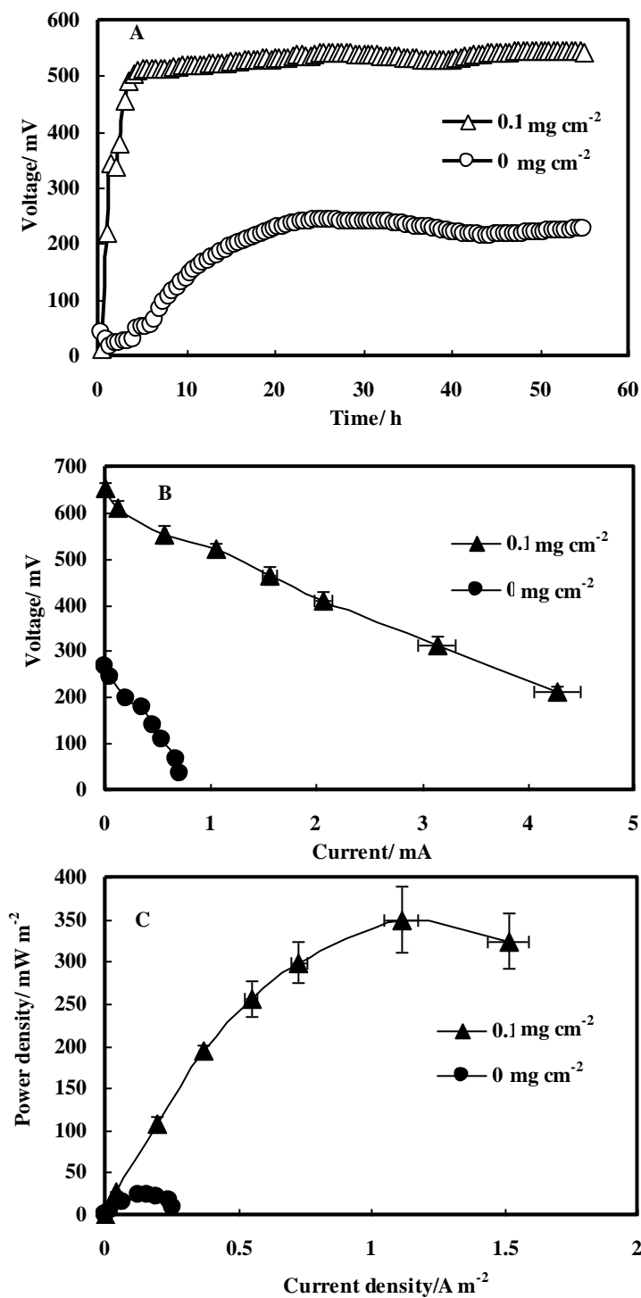
Figure 3. Effect of catalyst on function of the composting MFC. A: Voltage generation; B: Voltage-current curve; C: Power density curve. The error bars indicate standard deviation.
