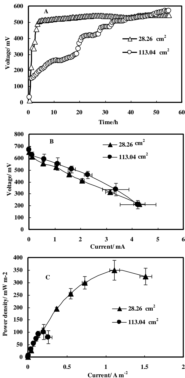
Figure 5. Effect of electrode area on performance of the composting MFC. A: Voltage generation; B: Voltage-current curve; C: Power density curve. The error bars indicate standard deviation.
