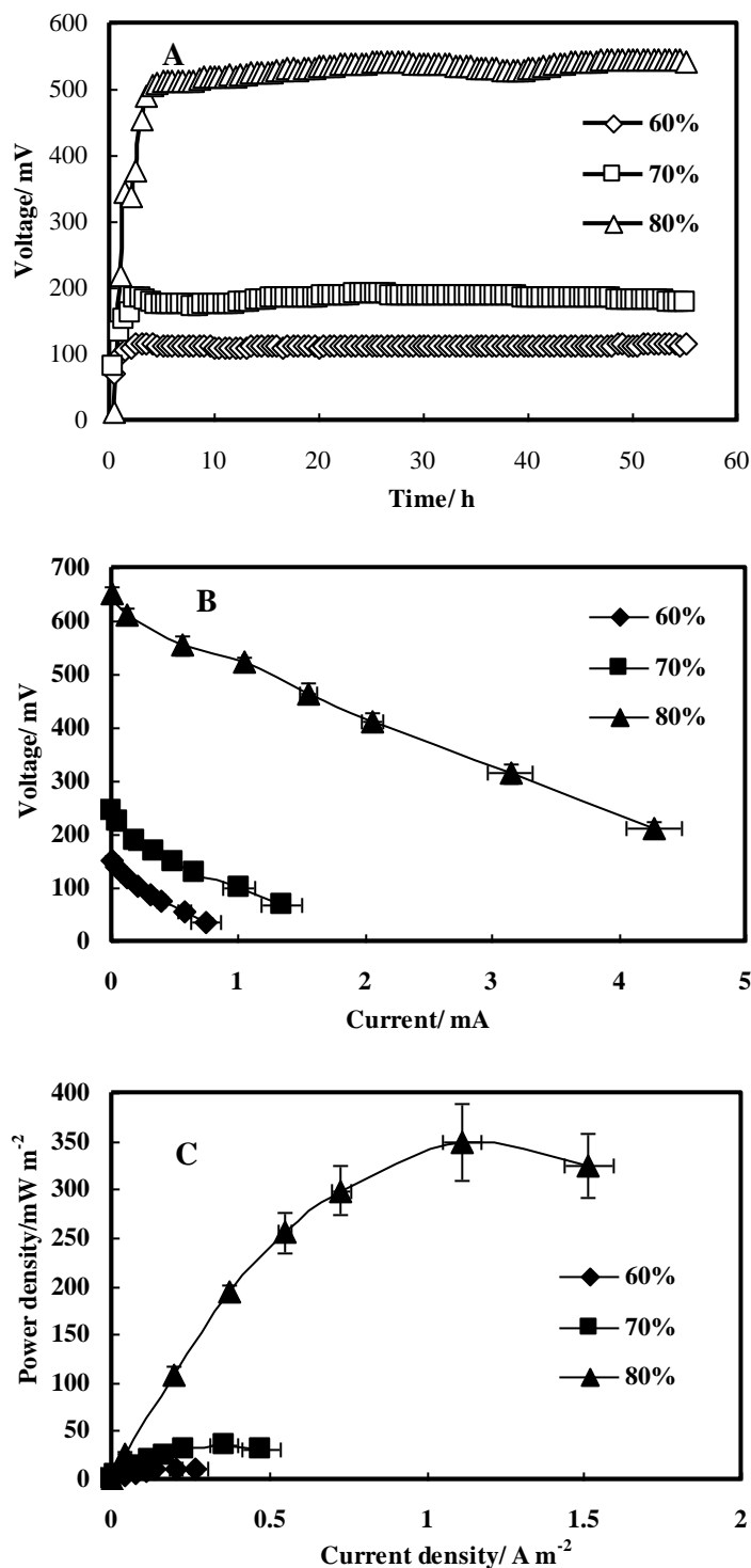
Figure 2. Effect of moisture content on performance of the composting MFC. A: Voltage generation; B: Voltage-current curve; C: Power density curve. The error bars indicate standard deviation.
