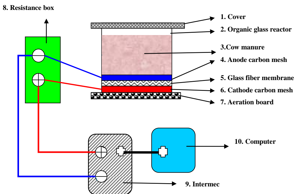
Figure 1. Schematic representation of the composting MFC system using cow manure as the substrate.
